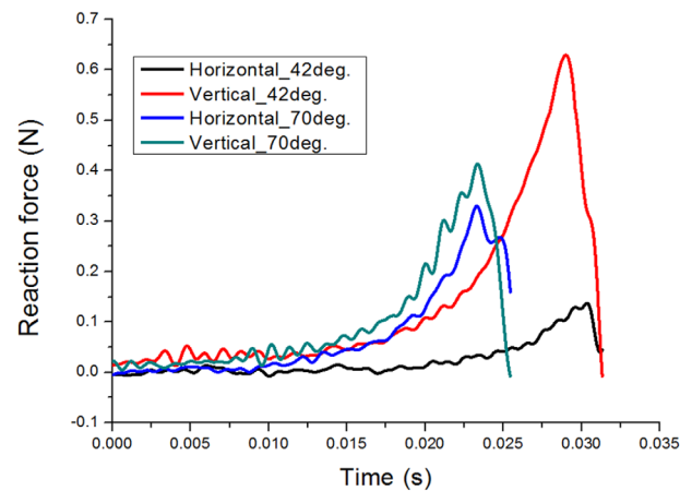
Figure 8. Measured ground reaction force for a leg stiffness of 0.0496 \text{ Nm rad}^{-1} and launch angles of 42^\circ and 70^\circ .
