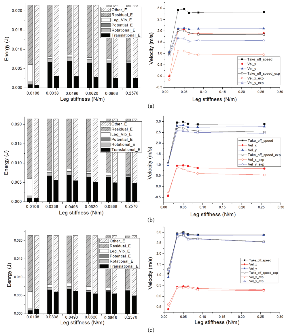
Figure 9. Energy distribution at take-off (left) and take-off velocity (right) with launch angles of (a) 70^\circ , (b) 54^\circ , and (c) 42^\circ . Note that the bars with bold border line represent the experimental data. The experiment measured only translational kinetic energy because of the difficulty of measuring the other energies.
