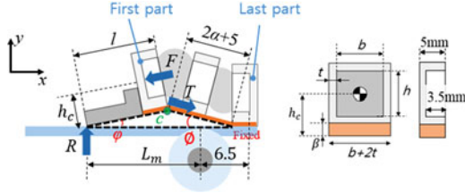
Fig. 9. FBD of the actuator module at 0° joint angle.
