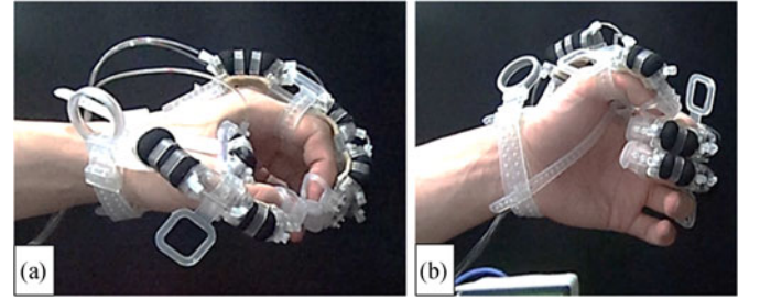
Fig. 15. Grasping posture. (a) General grasp, (b) Lateral pinch grasp.
