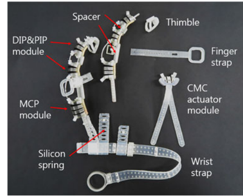
Fig. 3. Components of Exo-Glove PM.
