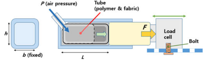
Fig. 7. Tube performance experiment setup.
